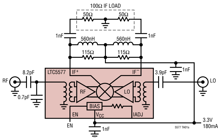
Wideband Downconverting Mixer with 1GHz IF Bandwidth and +15dBm Input P1dB into 100\Omega Load
