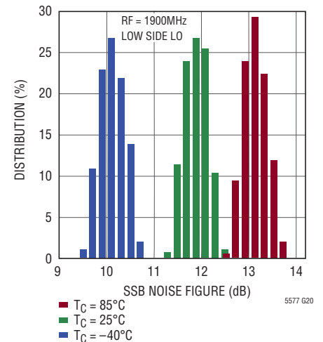
1900MHz SSB NF Distribution
