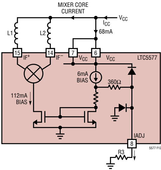
Figure 12. IADJ Interface
