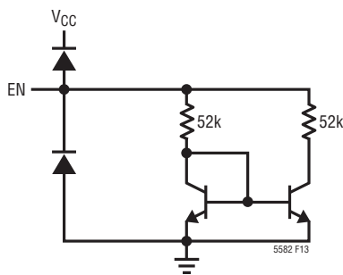
Figure 13. Enable Pin Simplified Circuit
