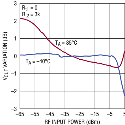
Output Voltage Temperature Variation from 25°C, 5800MHz
