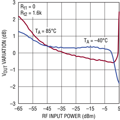
Output Voltage Temperature Variation from 25°C, 2700MHz
