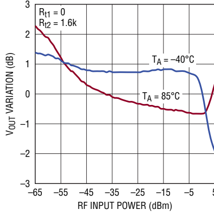
Output Voltage Temperature Variation from 25°C, 3800MHz
