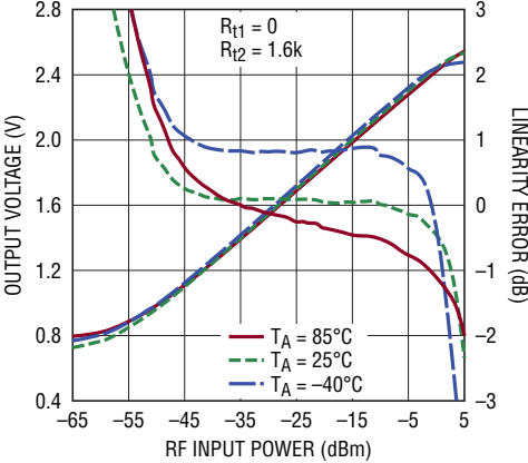
Output Voltage, Linearity Error vs RF Input Power, 3800MHz
