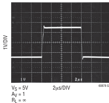
Large-Signal Response
