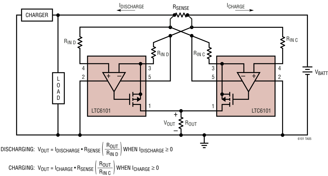
Bidirectional Current Sense Circuit with Combined Charge/Discharge Output
