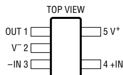
S5 PACKAGE 5-LEAD PLASTIC TSOT-23 T_{JMAX} = 150^\circ C , \theta_{JA} = 250^\circ C/W
