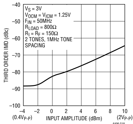
Differential Intermodulation Distortion vs Input Amplitude
