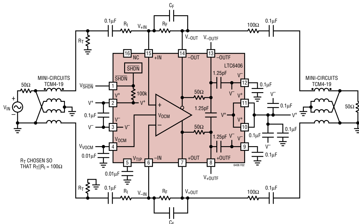
Figure 2. AC Test Circuit (–3dB BW testing)
