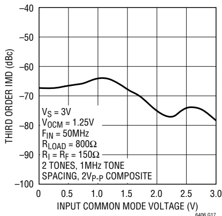
Differential Intermodulation Distortion vs Input Common Mode Voltage
