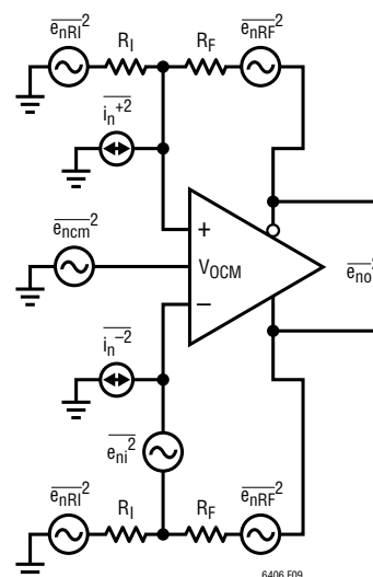
Figure 9. Noise Model of the LTC6406
