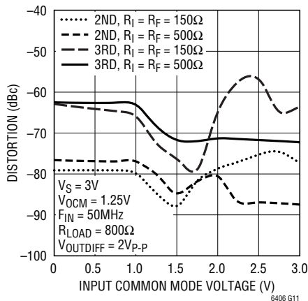
Single-Ended Harmonic Distortion vs Input Common Mode Voltage
