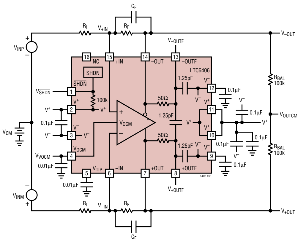
Figure 1. DC Test Circuit
