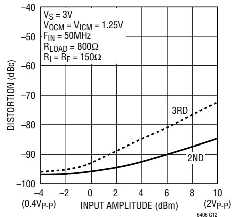
Differential Harmonic Distortion vs Input Amplitude
