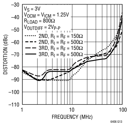
Single-Ended Harmonic Distortion vs Frequency
