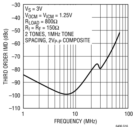
Differential Intermodulation Distortion vs Frequency
