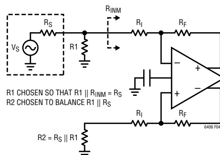
Figure 4. Optimal Compensation for Signal Source Impedance
