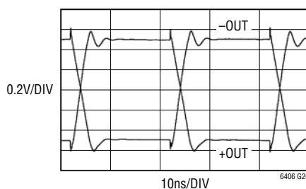
Large Signal Step Response
