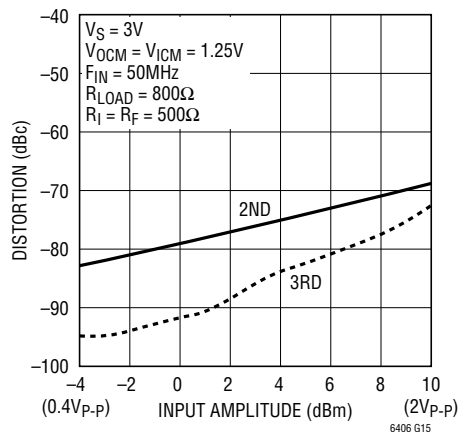
Single-Ended Harmonic Distortion vs Input Amplitude
