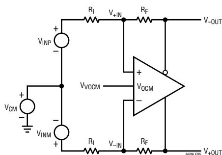
Figure 5. Circuit for Common Mode Range
