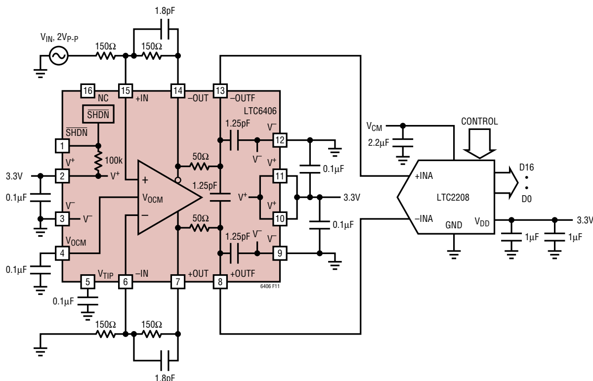
Figure 11. Interfacing the LTC6406 to an ADC
