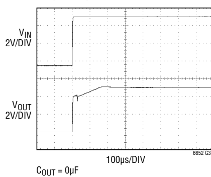
5V Start-Up Response Without Output Capacitor
