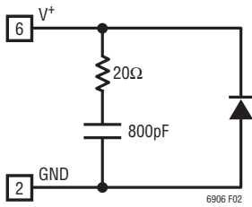
Figure 2. V+ Pin
