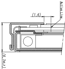
SECTION A-A' (S-5/1)
