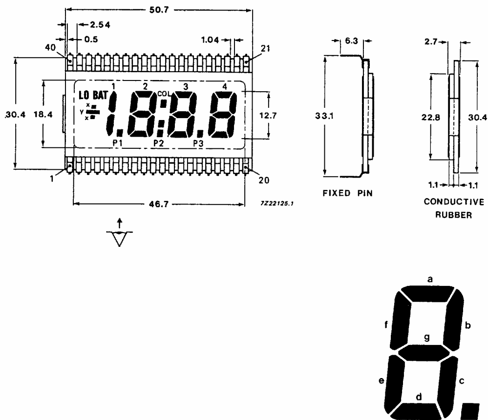
Fig.2 Display dimensions.
