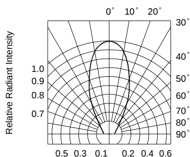
FIG.6 RADIATION DIAGRAM
