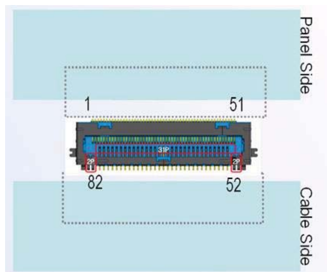
Fig. Connector diagram
