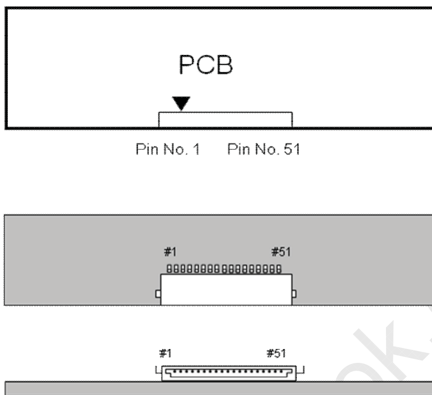
Fig. Connector diagram
