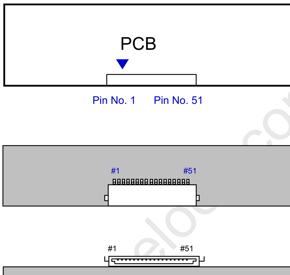
Fig. Connector diagram
