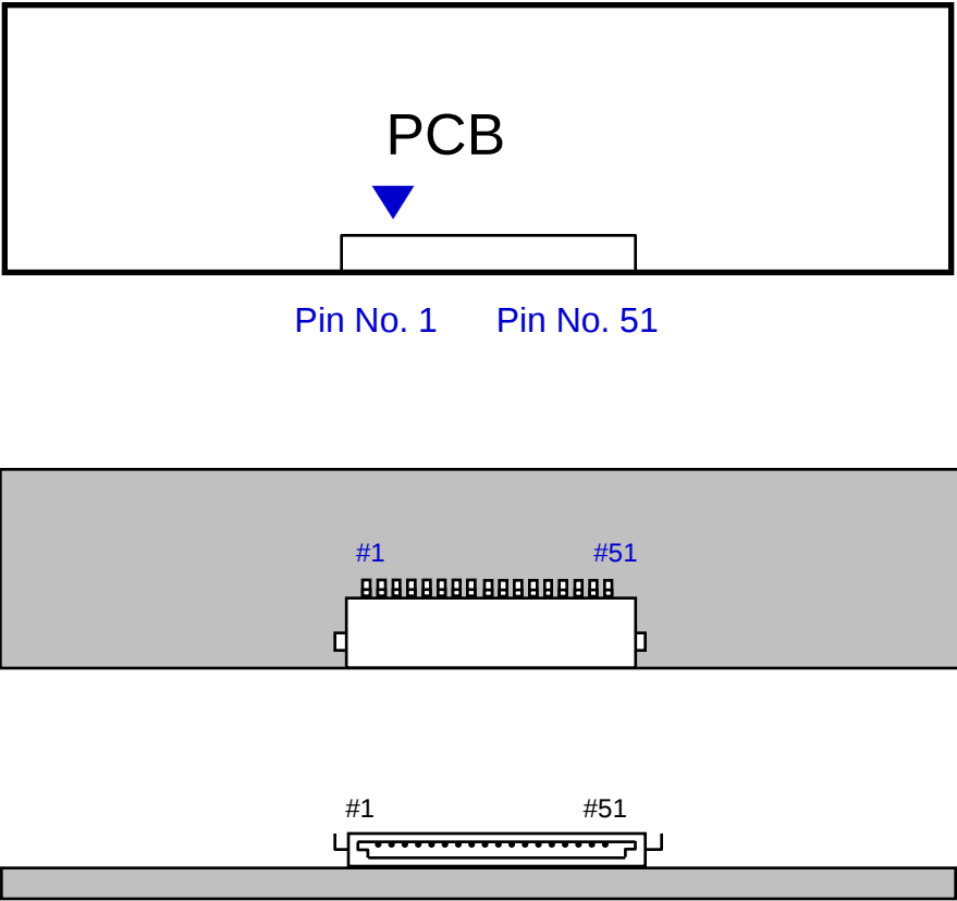
Fig. Connector diagram
