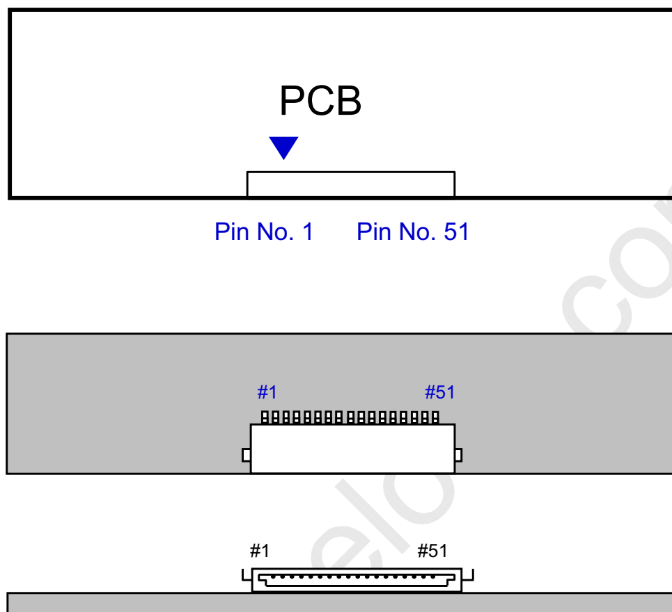
Fig. Connector diagram
