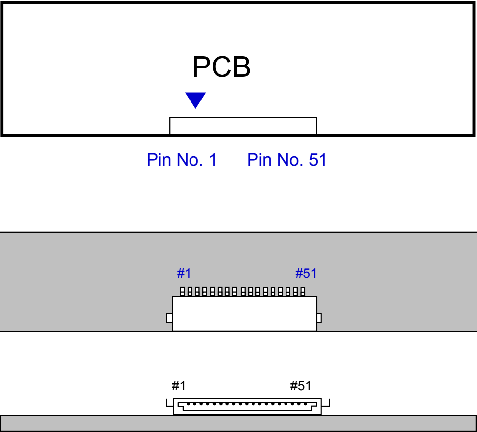
Fig. Connector diagram
