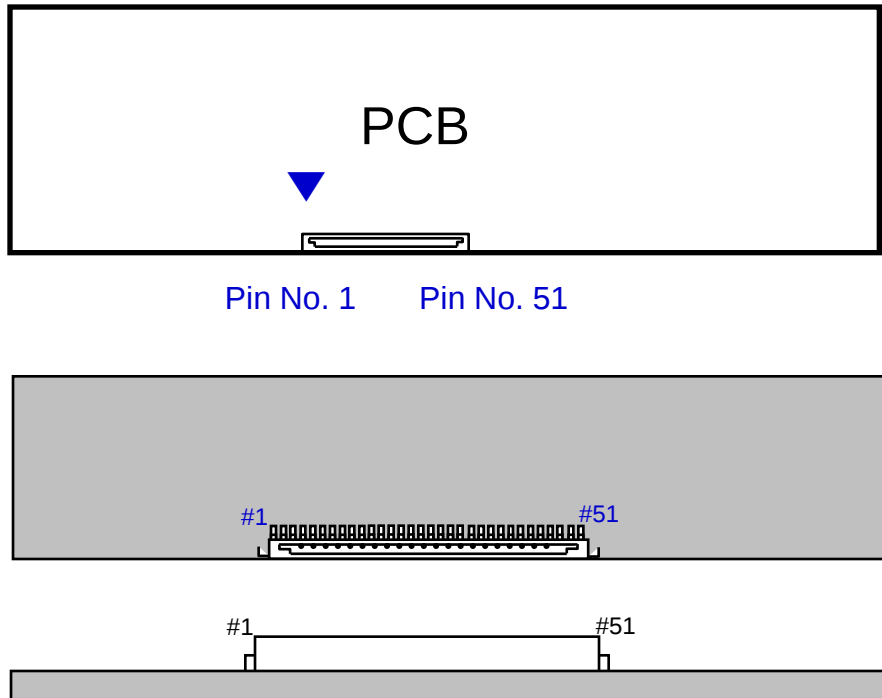
Fig. Connector diagram
