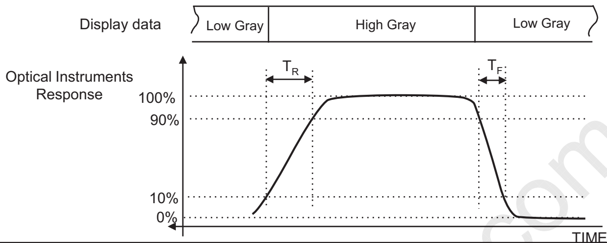
Gray to Gray Response Time
