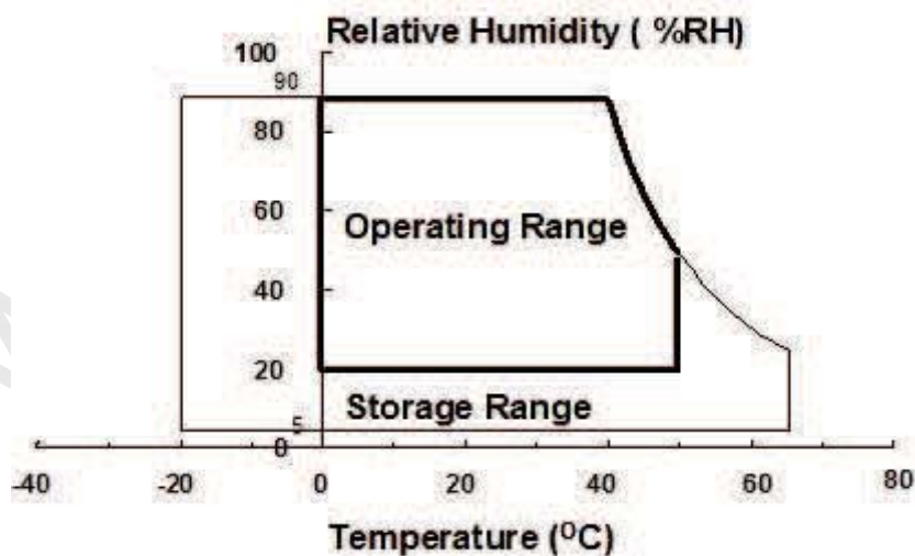
Fig. Temperature and Relative humidity range
