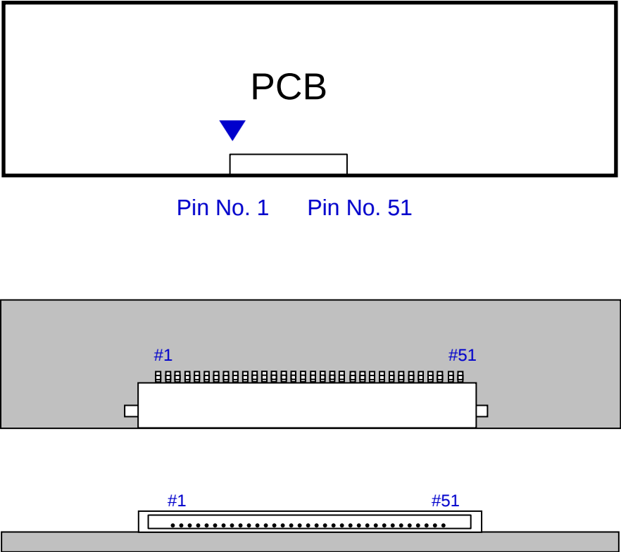
Fig. Connector diagram
