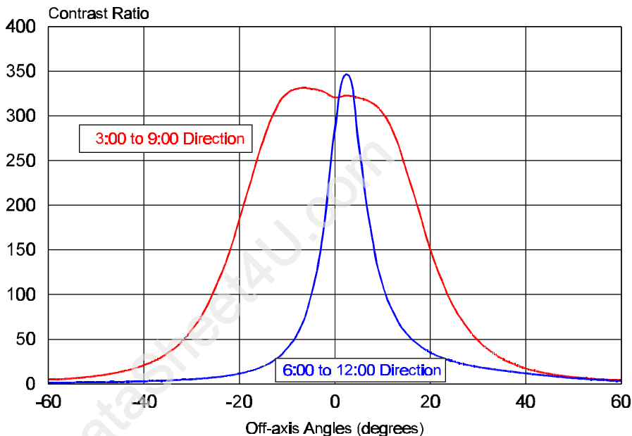
LM130A-12C318 LCD Contrast Ratio Angular Distribution
