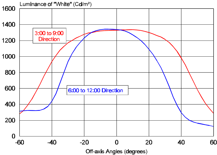
LM130A-12C318 LCD Screen Brightness Angular Distribution
