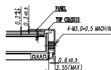
SECTION A-A(S:3/1) (SIDE MOUNT HOLE)
