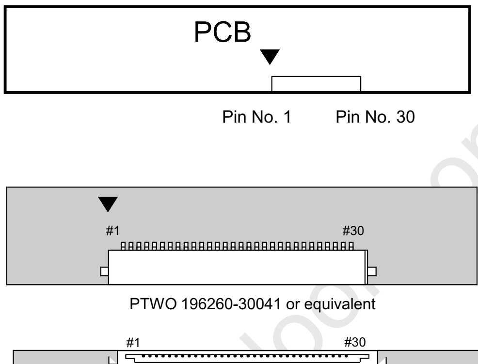
Fig. Connector diagram
