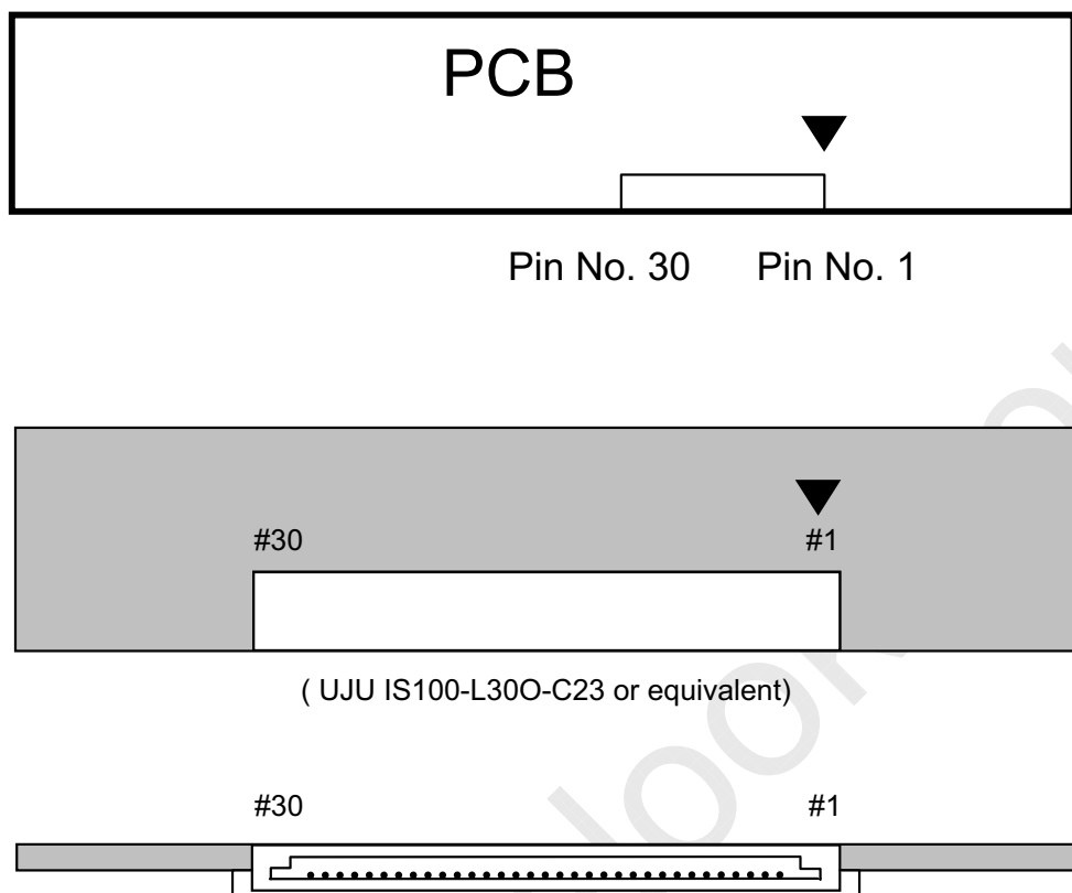
Fig. Connector diagram
