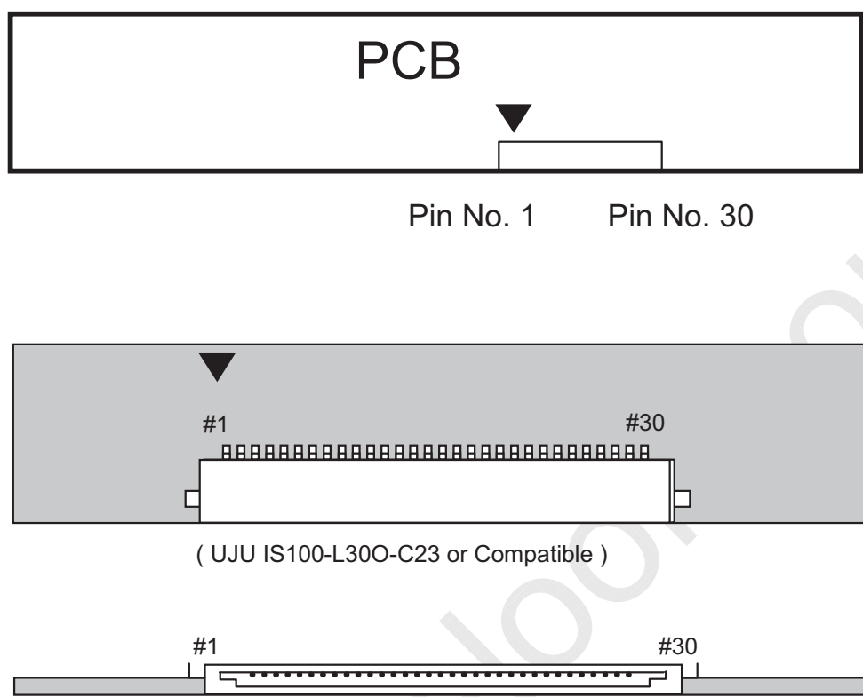
Fig. Connector diagram
