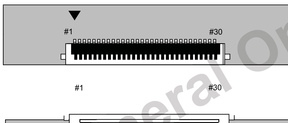
Fig. Connector diagram
