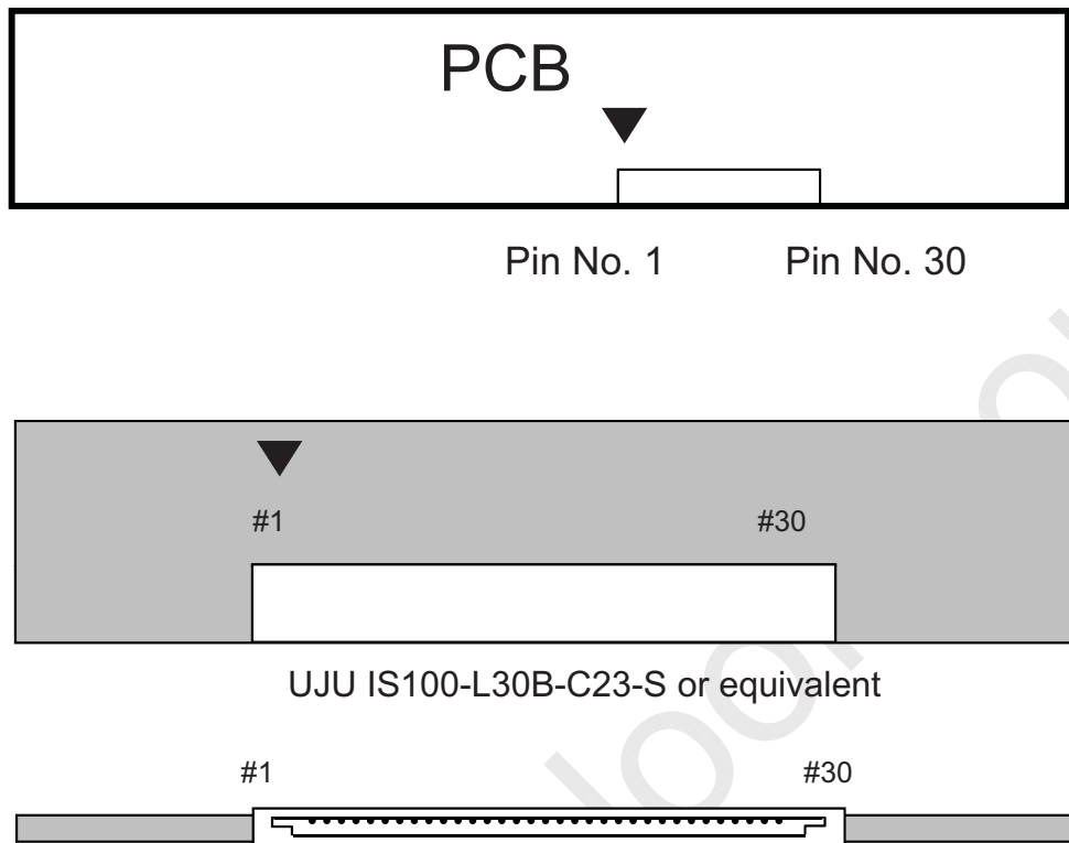
Fig. Connector diagram
