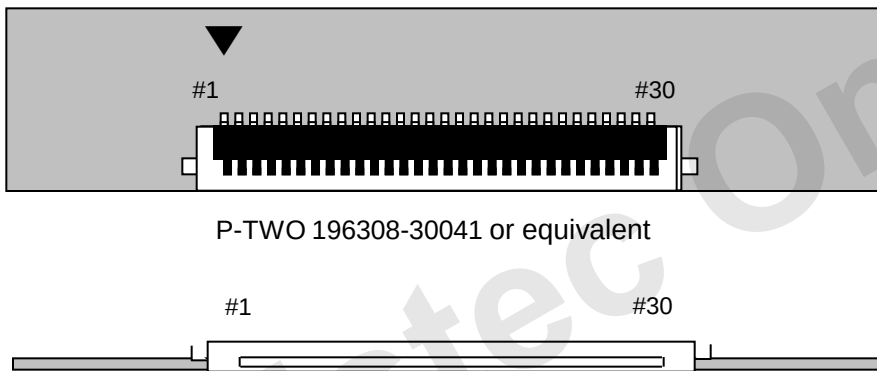
Fig. Connector diagram
