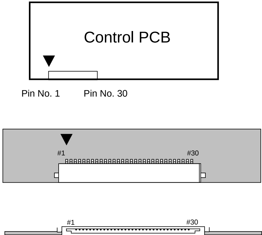
Fig. Connector diagram
