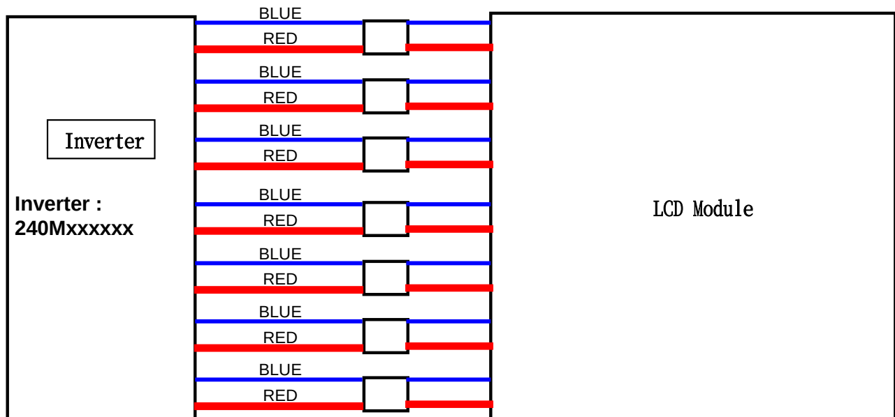
Fig. Measurement point of Lamp Current
