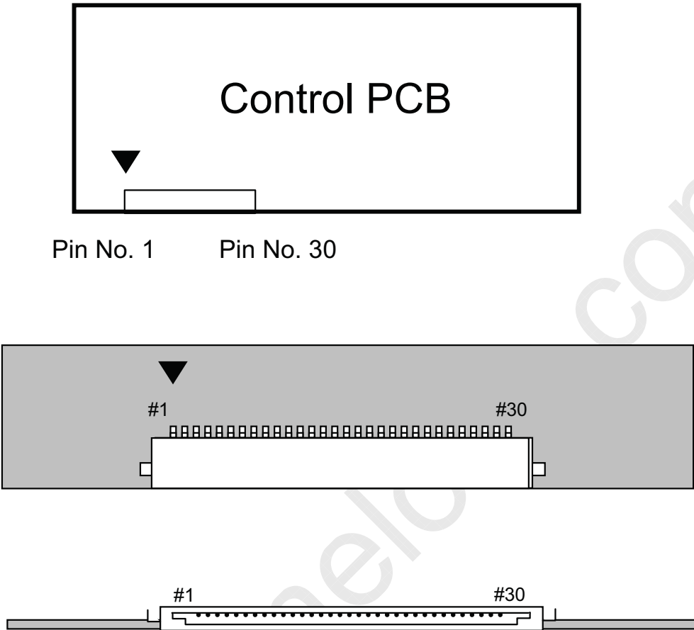
Fig. Connector diagram
