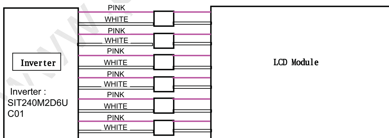
Fig. Measurement point of Lamp Current
