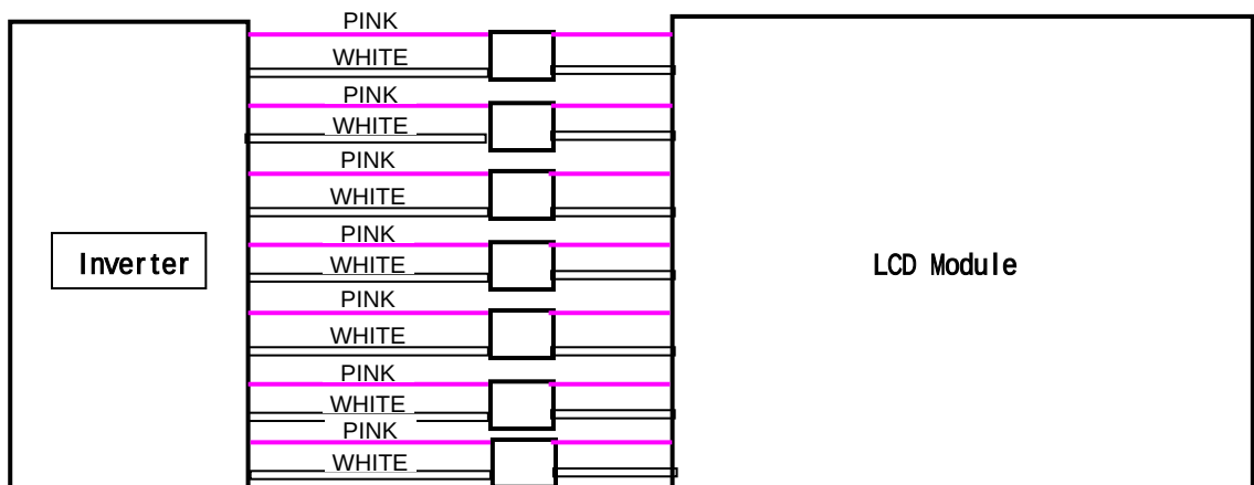
Fig. Measurement point of Lamp Current
