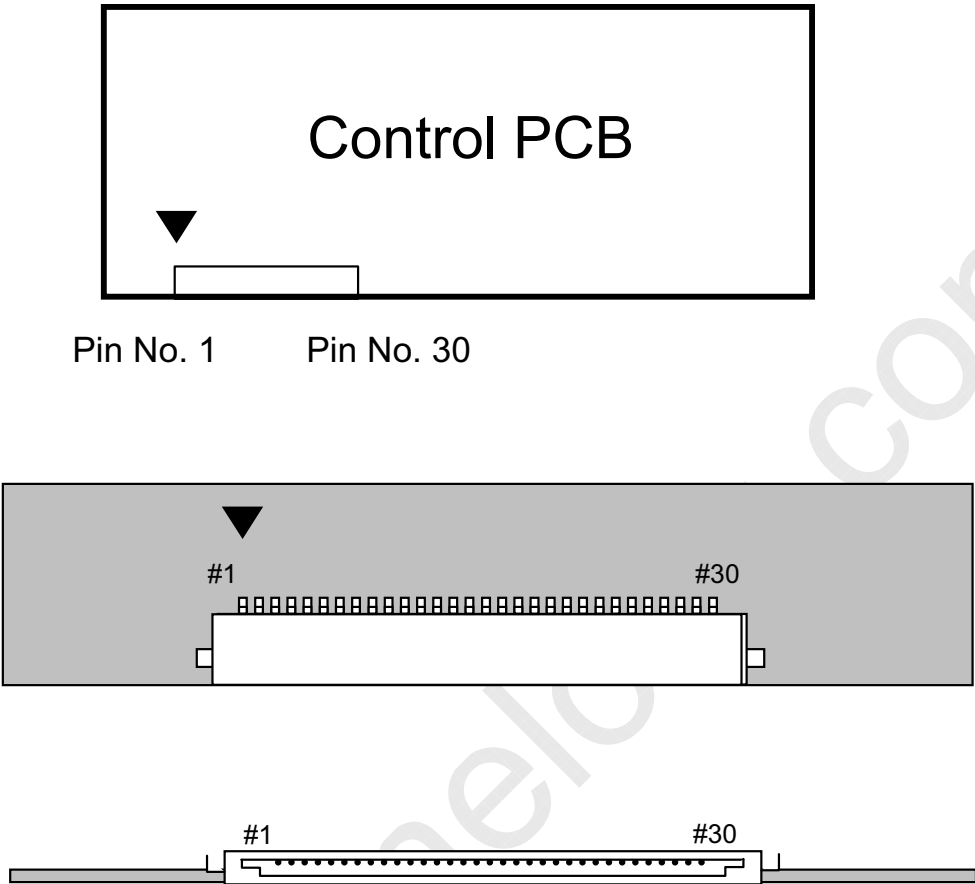
Fig. Connector diagram
