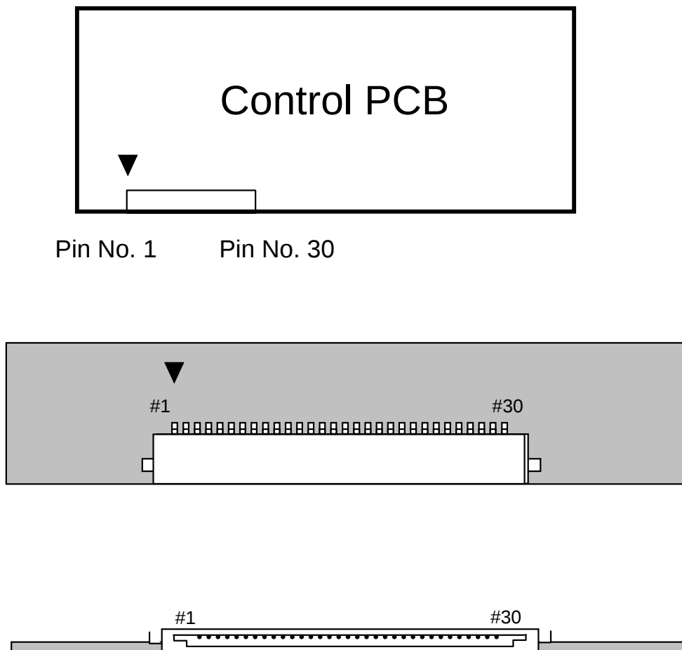
Fig. Connector diagram
