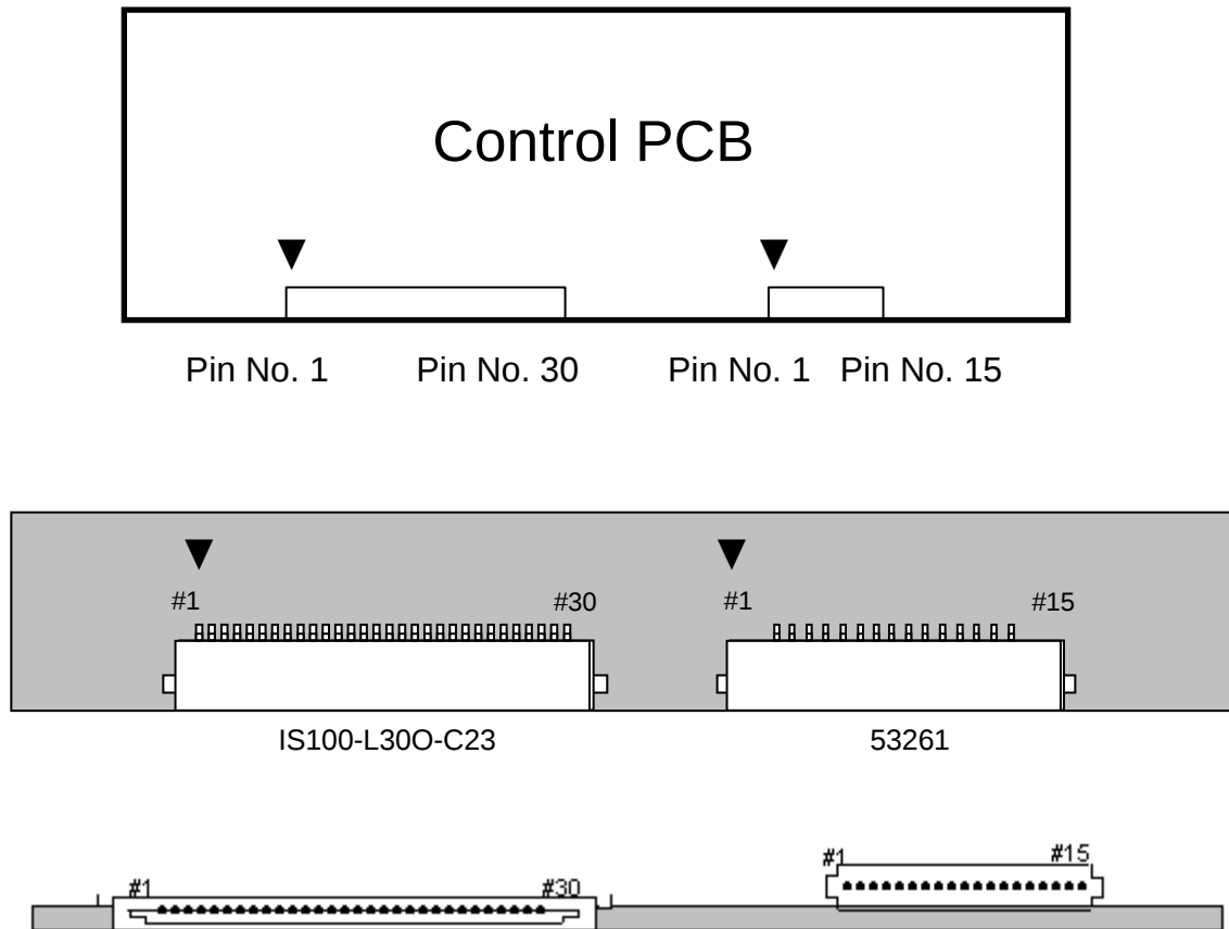
Fig. Connector diagram
