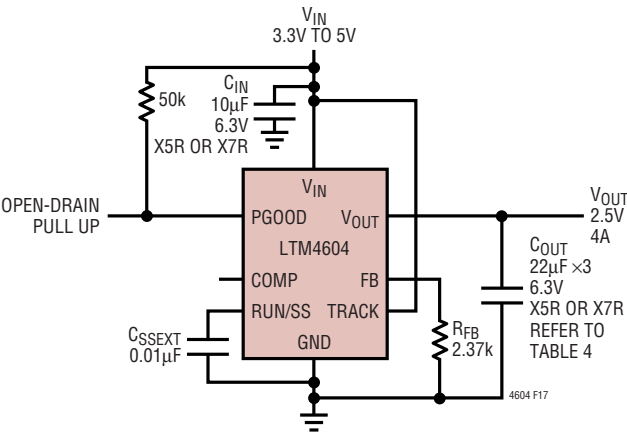
Figure 17. 3.3V to 5V Input, 2.5V at 4A Design
