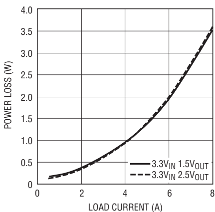
Figure 7. 3.3V IN , 2.5V OUT and 1.5V OUT Power Loss
