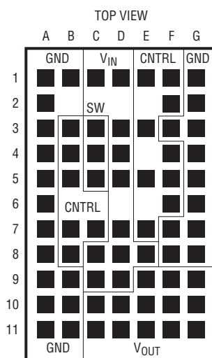
LGA PACKAGE 68-PIN (15mm × 9mm × 2.8mm)
