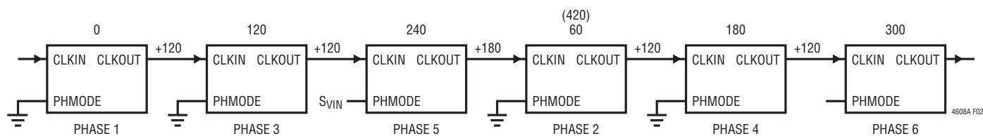
Figure 2. 6-Phase Operation
