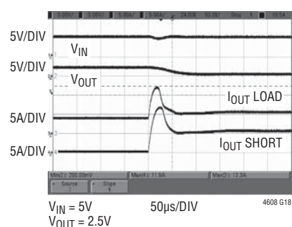
Short-Circuit Protection (2.5V Short, 4A Load)
