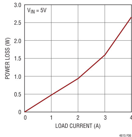
Figure 6. 3.3V Power Loss
