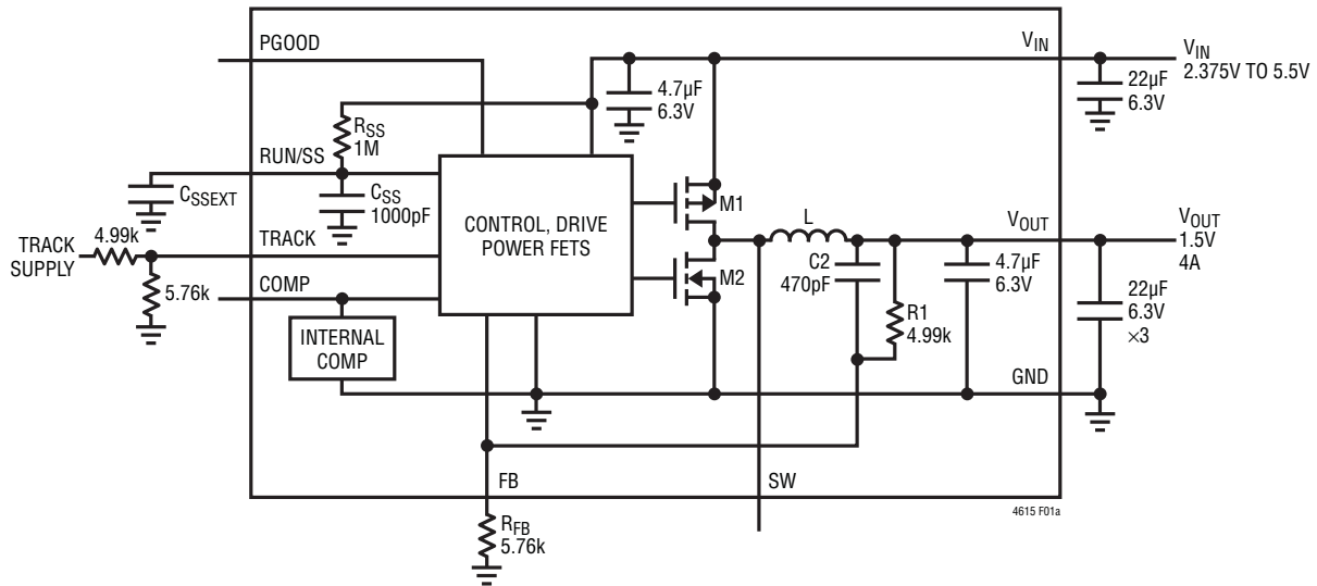
VLDO Block Diagram
