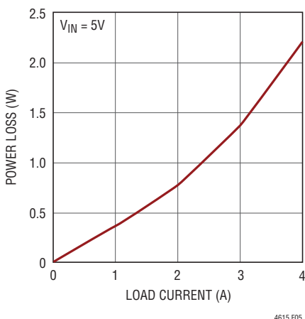
Figure 5. 1.2V Power Loss
