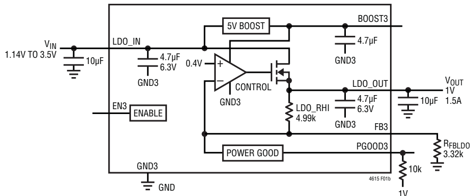
Figure 1. Simplified LTM4615 Block Diagram of Each Switching Regulator Channel and the VLDO
