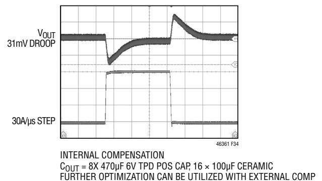
Figure 33. 12V to 0.9V 30A/μs Load Step
