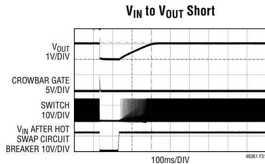
Figure 31. 12V to 0.9V Overvoltage Trip
