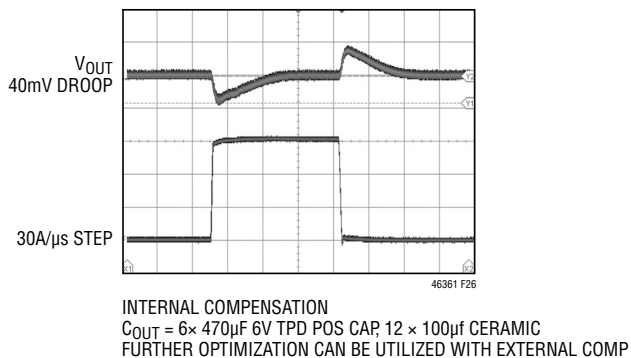
Figure 26. 12V to 0.9V 30A/μs Load Step
