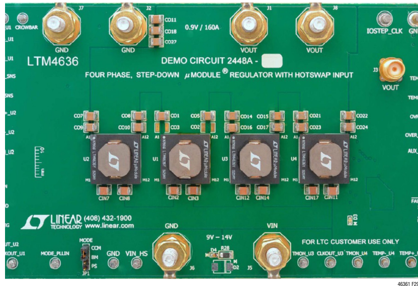
Figure 29. DC2448A Demo Board
