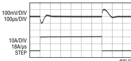
2.5V Transient Response
