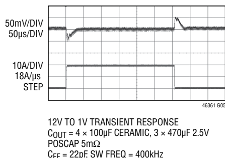
1V Transient Response
