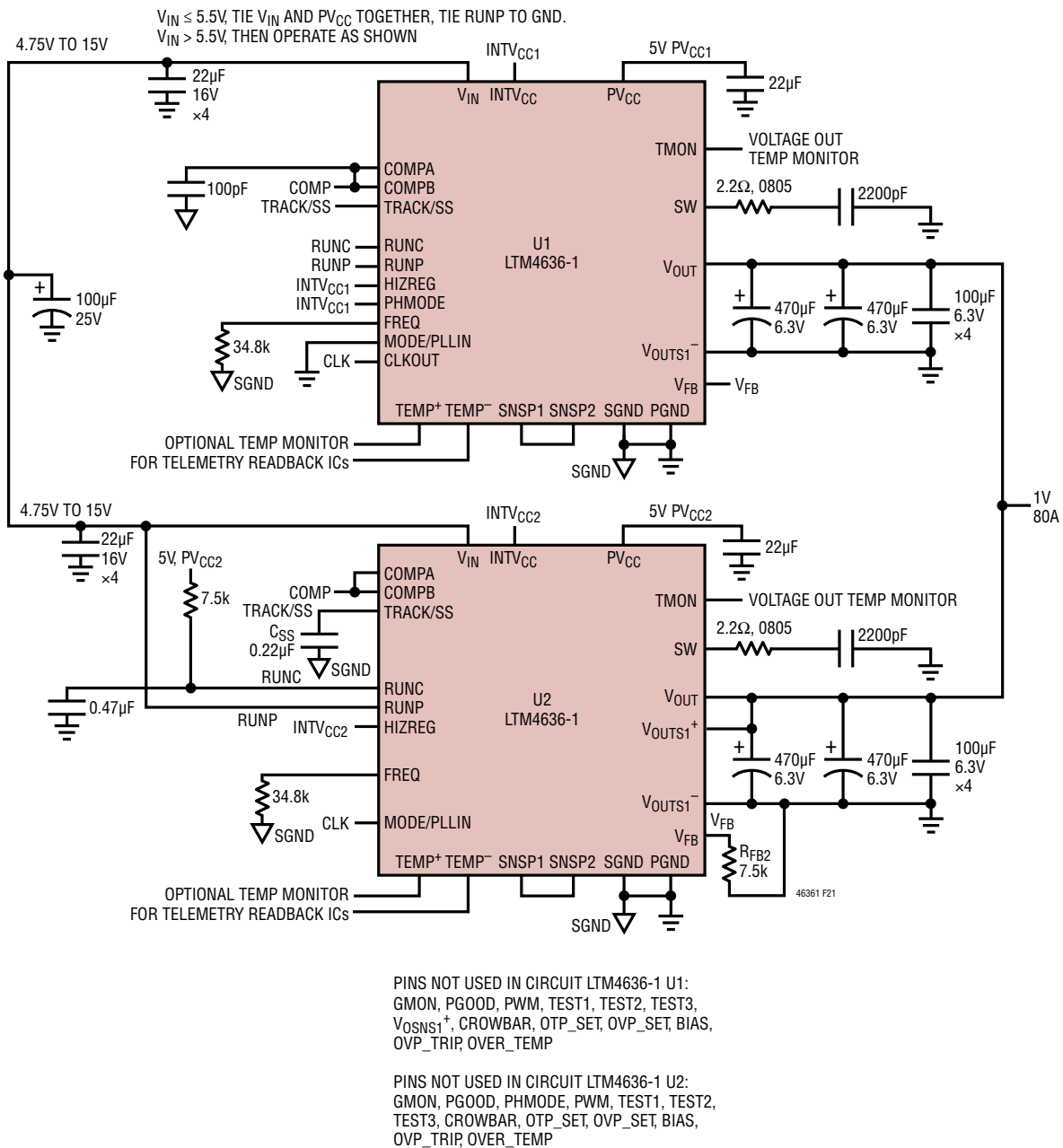
Figure 21. 2-Phase 1V, 80A Regulator Design
