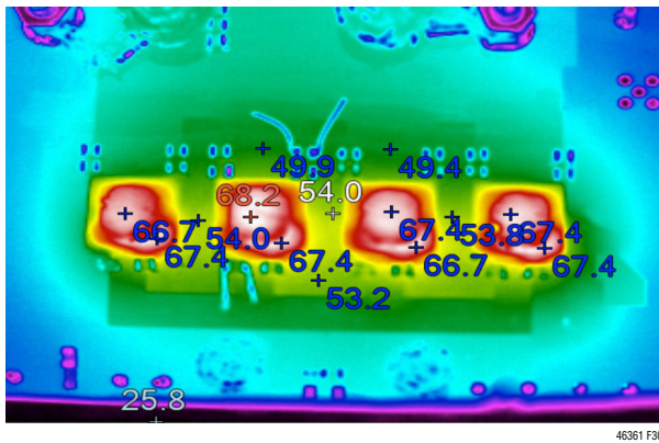
Figure 30. Thermal Plot, 12V to 0.9V at 160A, 400LFM Air Flow
