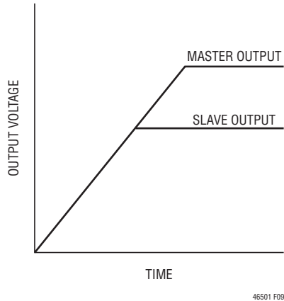
Figure 9. Output Coincident Tracking Waveform
