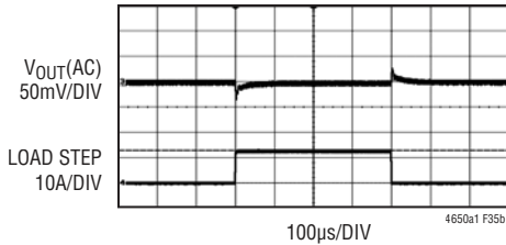
25% Load Step Transient Response ±3% Output Regulation Window. 12VIN, 1.0VOUT, 50A per Above Circuit
