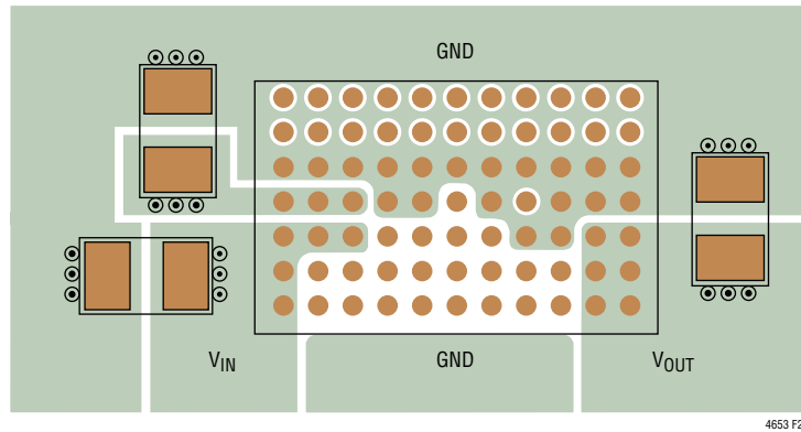
Figure 29. Recommend PCB Layout, Package Top View
