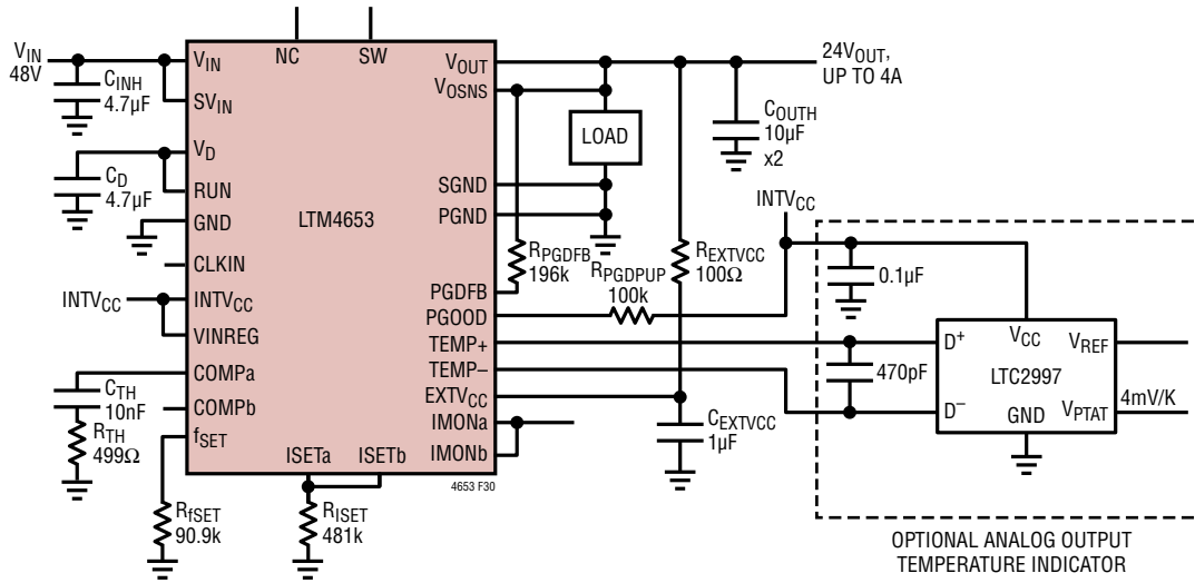
Figure 30. 4A, 24V Output DC/DC \mu Module Regulator
