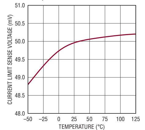
Current Limit Voltage vs Temperature
