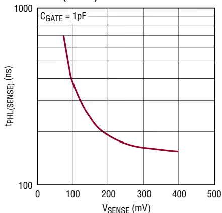
Current Limit Propagation Delay ( t_{\text{PHL(SENSE)}} ) vs V_{\text{SENSE}}
