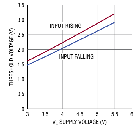
Logic Input Threshold vs V_L Supply Voltage
