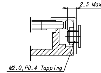
SECTION A-A' (S=5/1)
