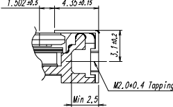
SECTION B-B' (S=4/1)
