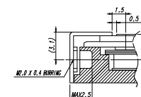
SECTION D-D' (S:5/1)
