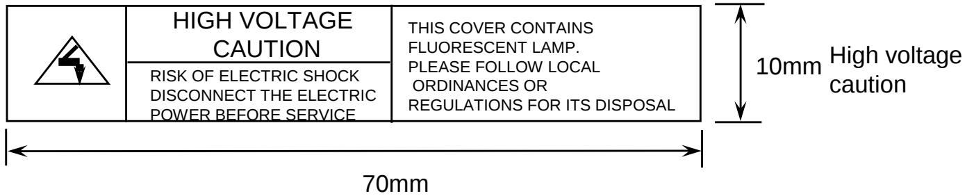
High voltage caution label
