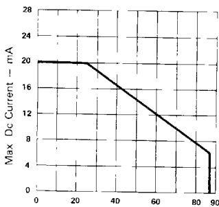
Fig 4 MAX ALLOWABLE DC CURRENT PFR SEG Vs AMBIENT TEMPERATURE
