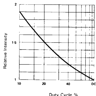
Fig 6 LUMINOUS INTENSITY Vs DUTY CYCLE % (AVERAGE I_v = 10 \text{ mA PER SEG} )
