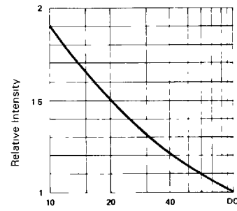
Fig 6 LUMINOUS INTENSITY VS DUTY CYCLE% (AVERAGE I_v - 10mA PER SEG)
