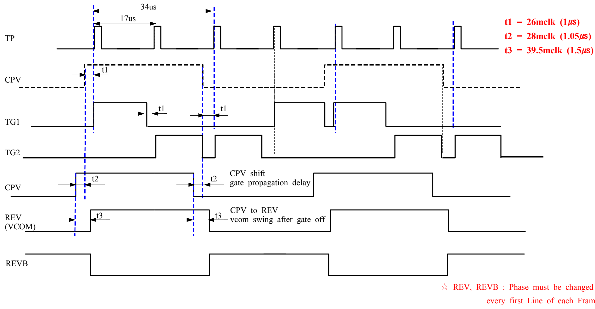
< Horizontal & Vertical Timing Diagram >
